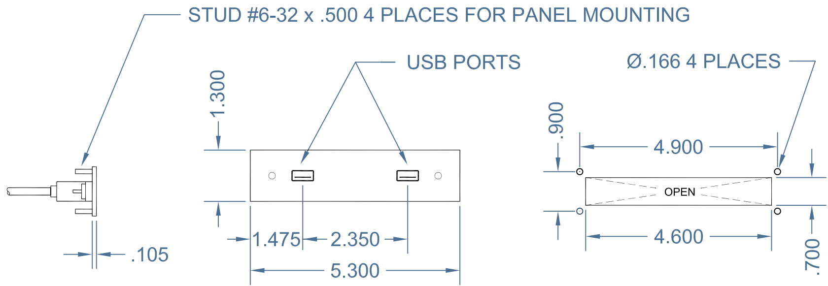
SIDE VIEW
