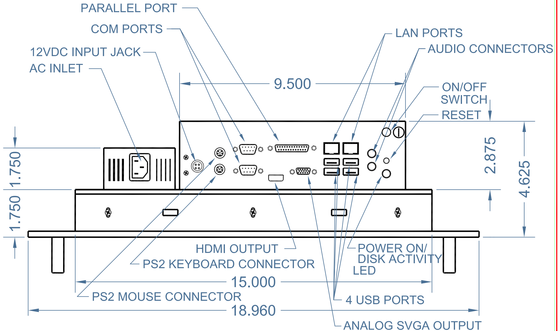
BOTTOM VIEW
