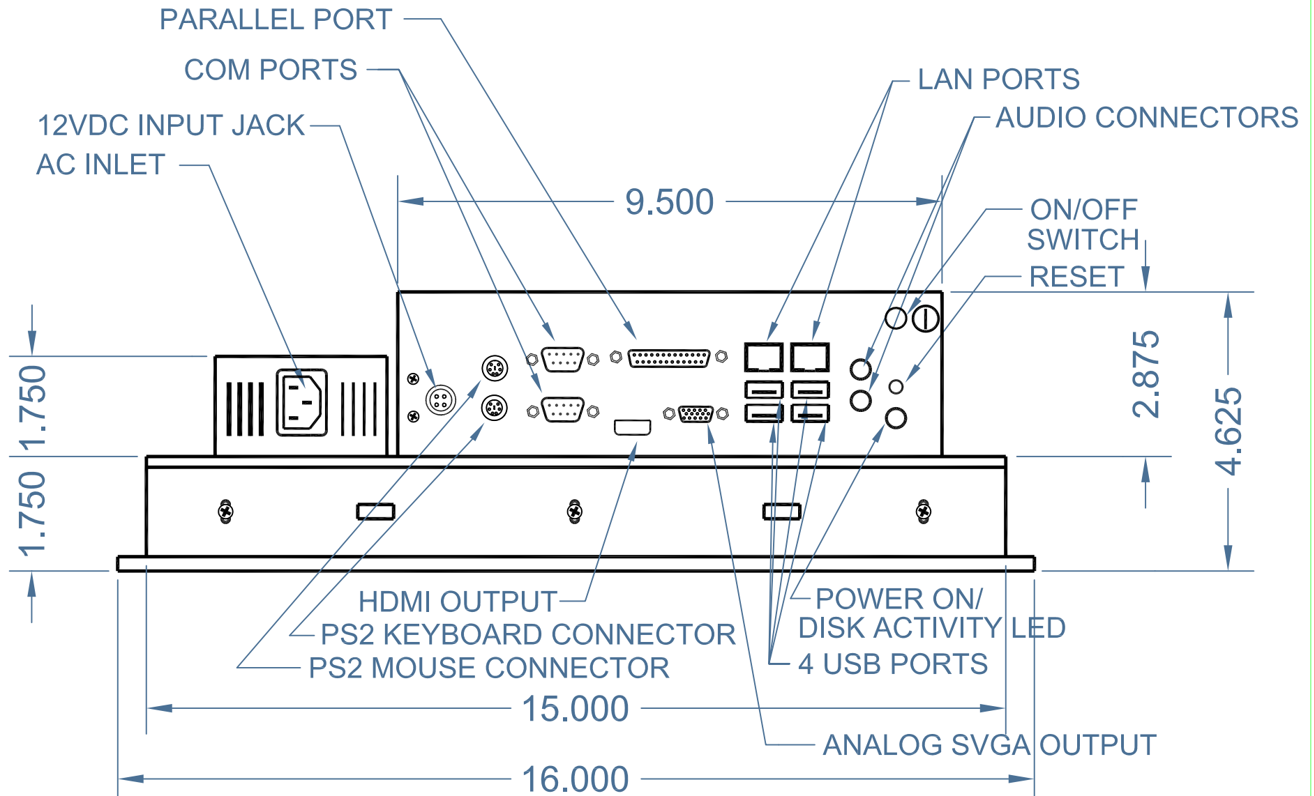
BOTTOM VIEW
