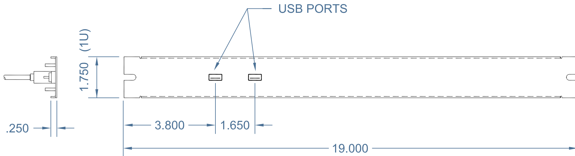
SIDE VIEW
