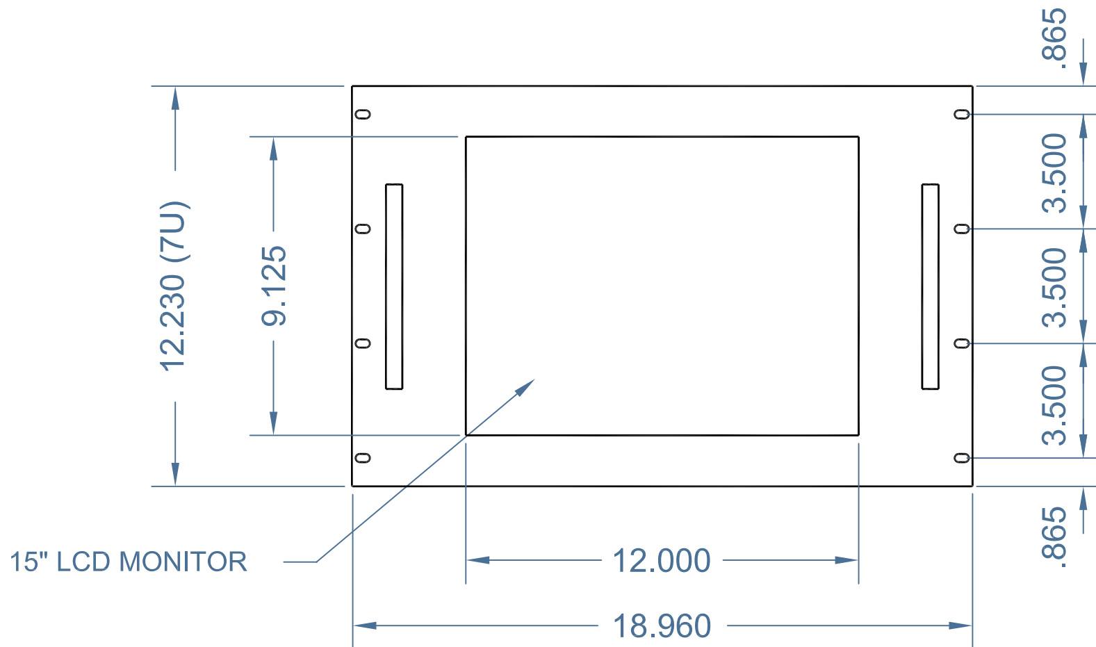
FRONT VIEW
