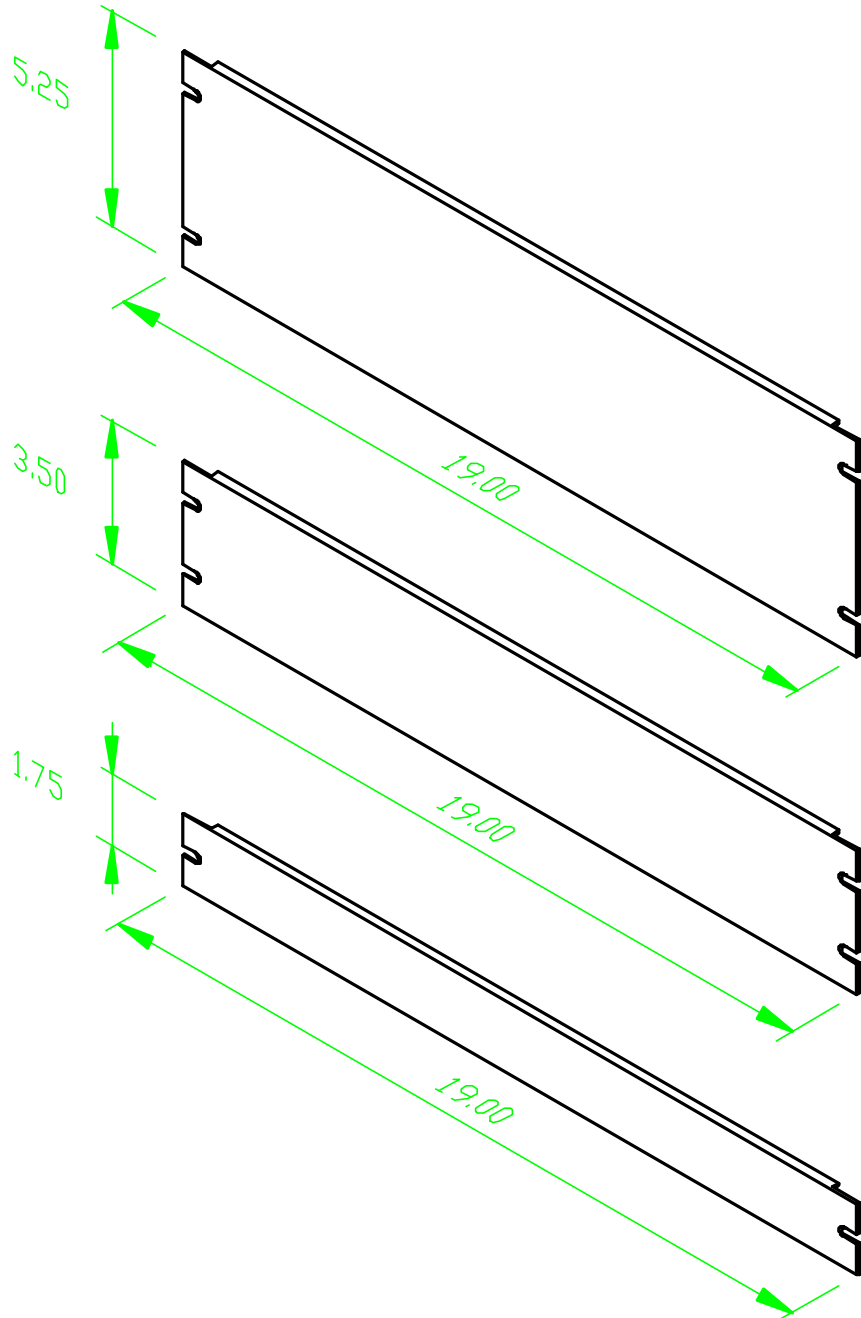
3U FILLER PANEL
